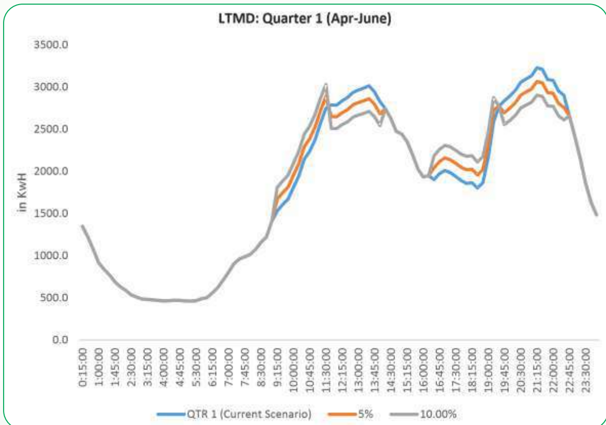
Figure 5-22: Change in LTMD load curve in Apr-May-June due to 5% and 10% load shift
