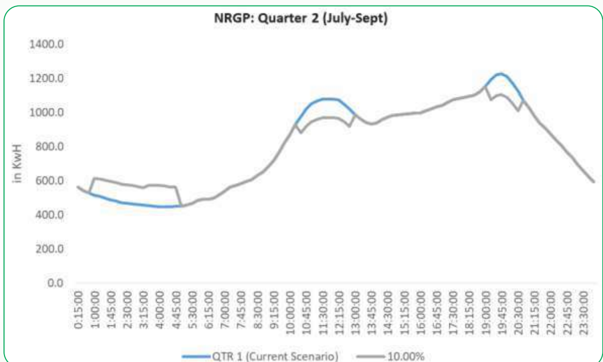
Figure 5-57: Change in NRGH night shift load curve in July-August-September due to 10% load shift
