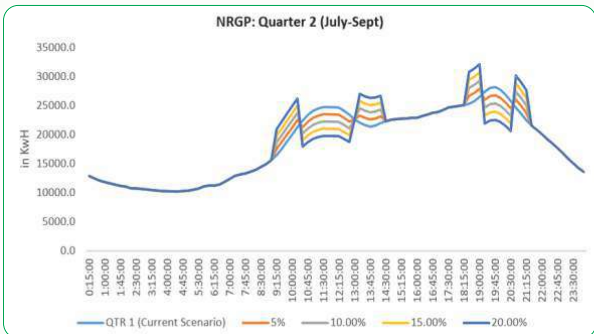
Figure 5-38: Change in NRG load curve in July-Aug-Sept due to 5%, 10%, 15% & 20% load shift
