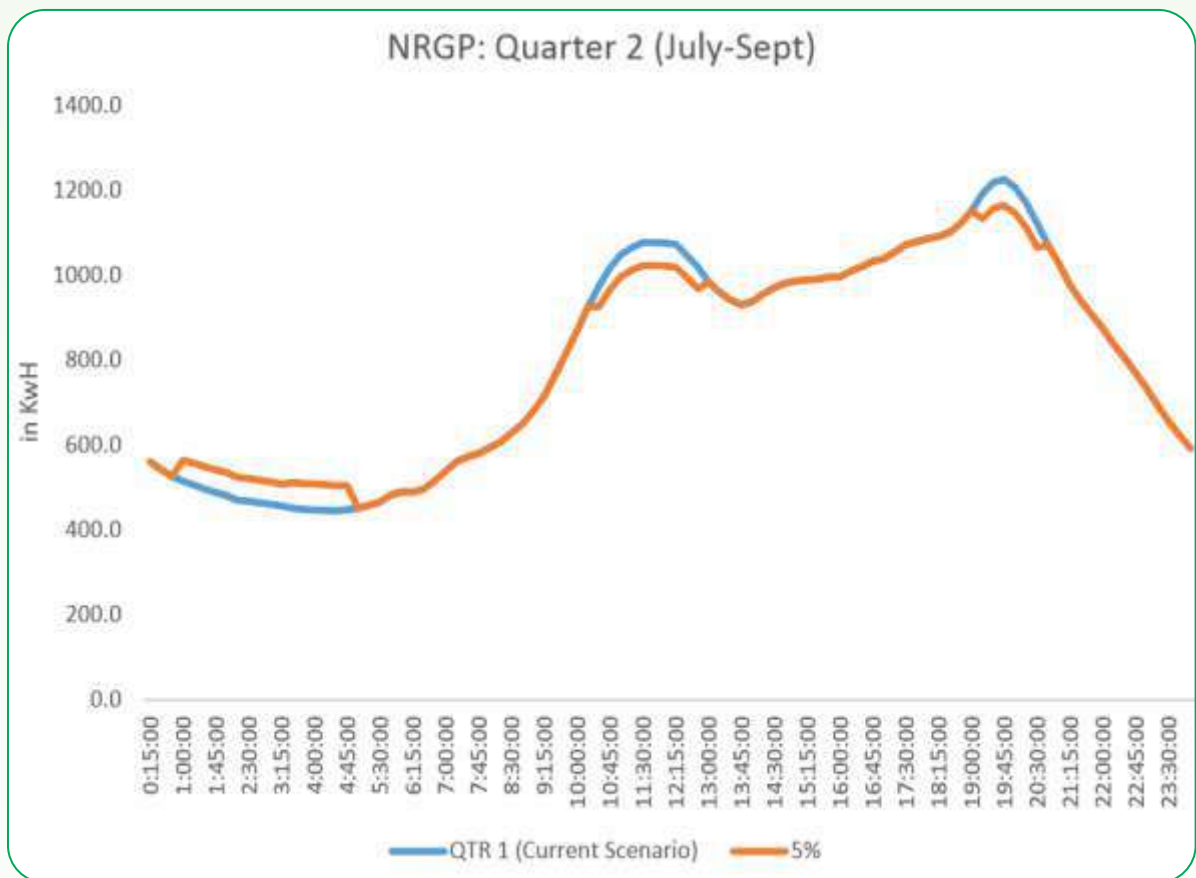
Figure 5-56: Change in NRGH night shift load curve in July-August-September due to 5% load shift
