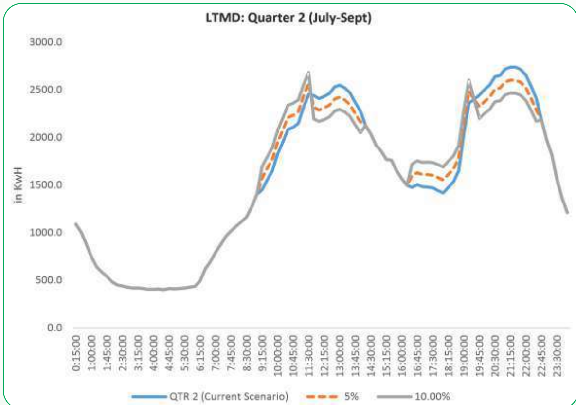
Figure 5-26: Change in LTMD load curve in July-Aug-Sept due to 5%, 10% load shift
