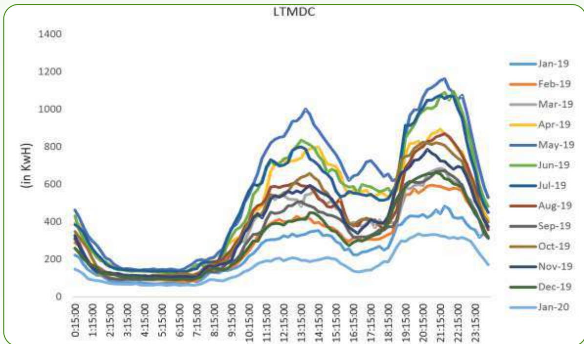
Figure 5-13: Consumption pattern for LTMDC consumers during Jan' 19- Jan' 20
