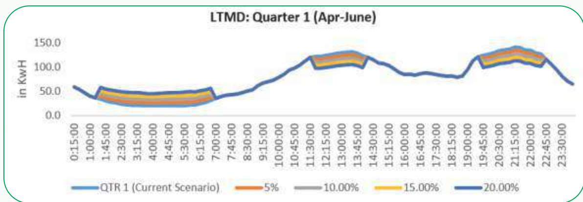
Figure 5-40: Load curve for LTMD night shift analysis consumers – First-quarter overall scenario
