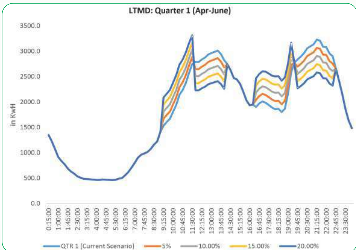
Figure 5-24: Change in LTMD load curve in Apr-May-June due to 5%, 10%, 15% and 20% load shift
