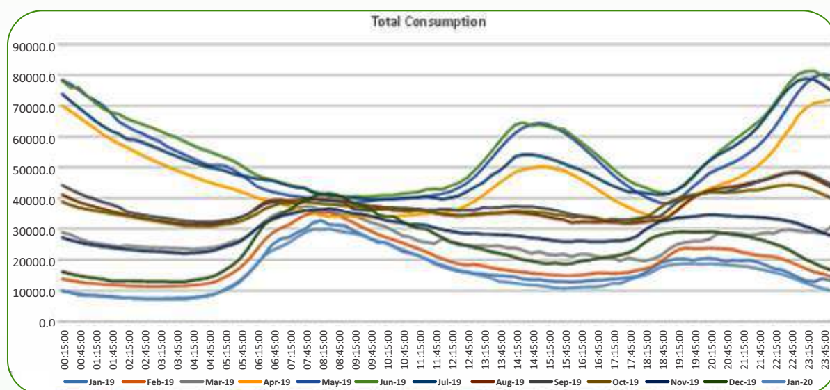
Figure 5-16: Total consumption pattern for all consumer in Naroda area (in KWh) (Jan-19 to Jan-20)
