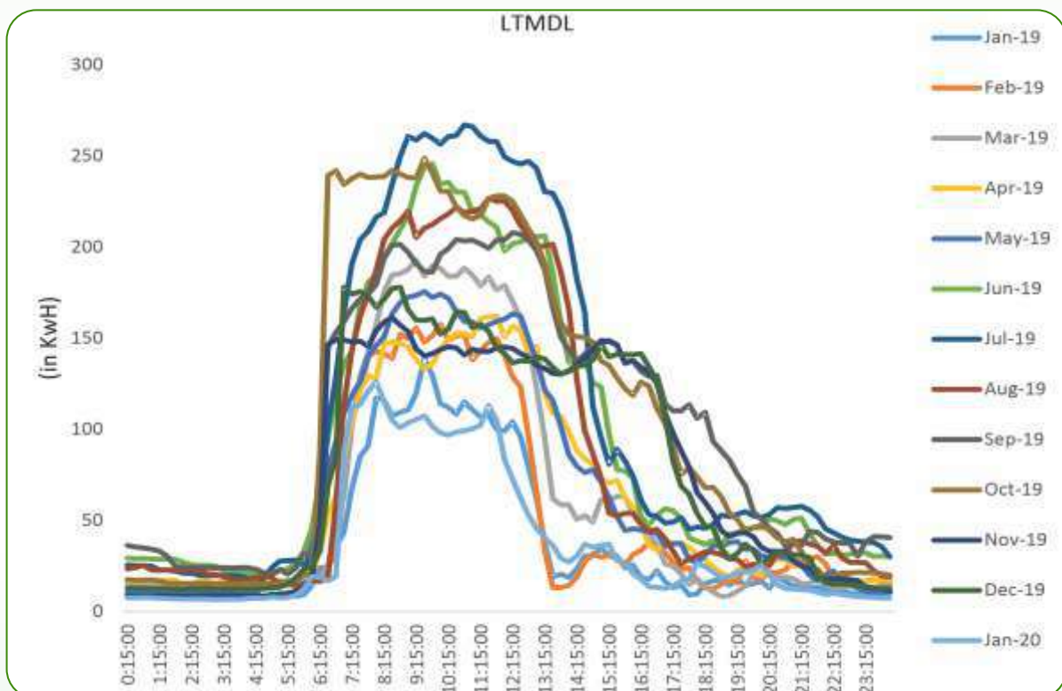
Figure 5-14: Consumption pattern for LTMDL consumers during Jan' 19- Jan' 20
