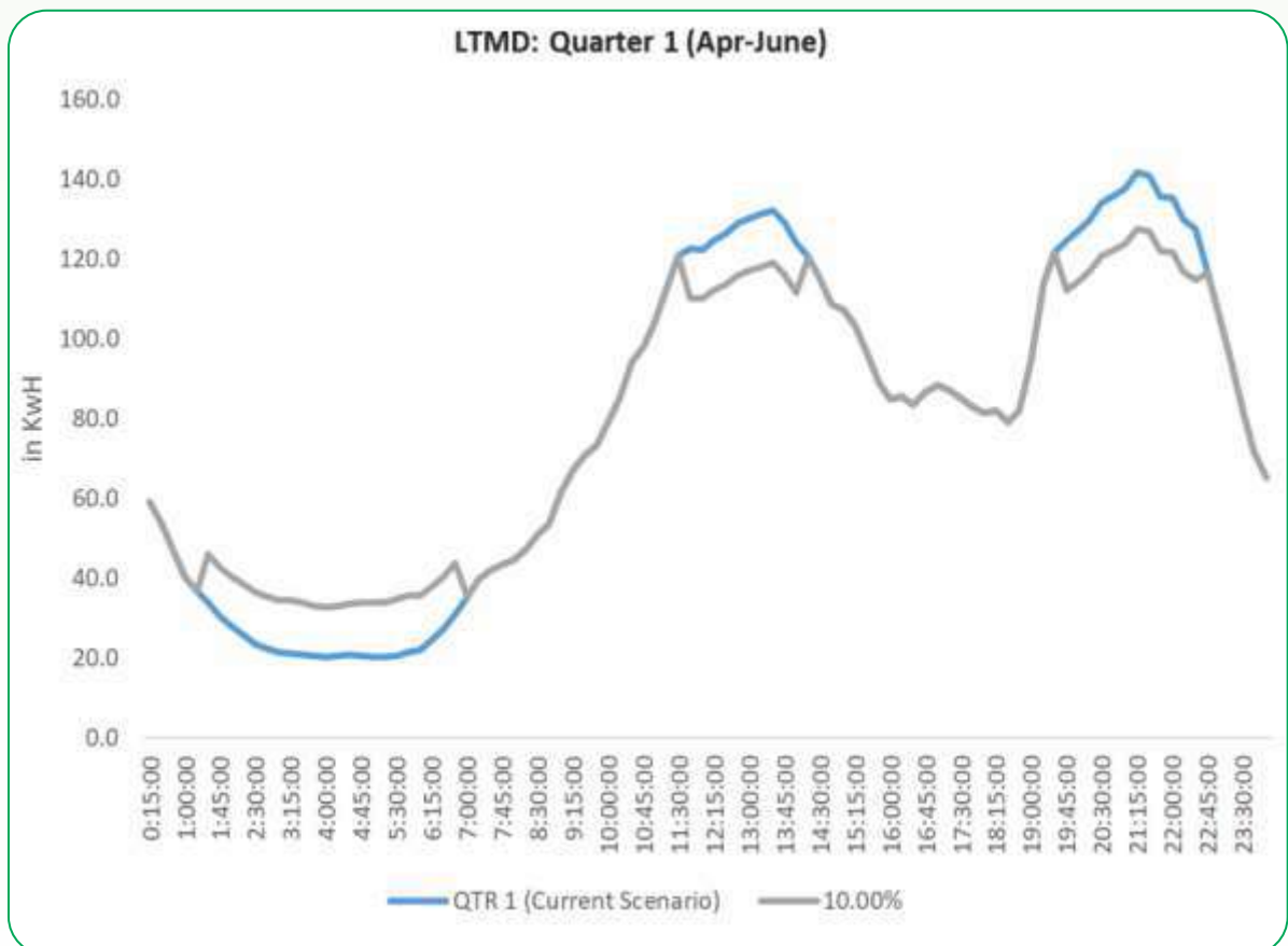
Figure 5-42: Change in LTMD night shift load curve in Apr-May-June due to 10% load shift
