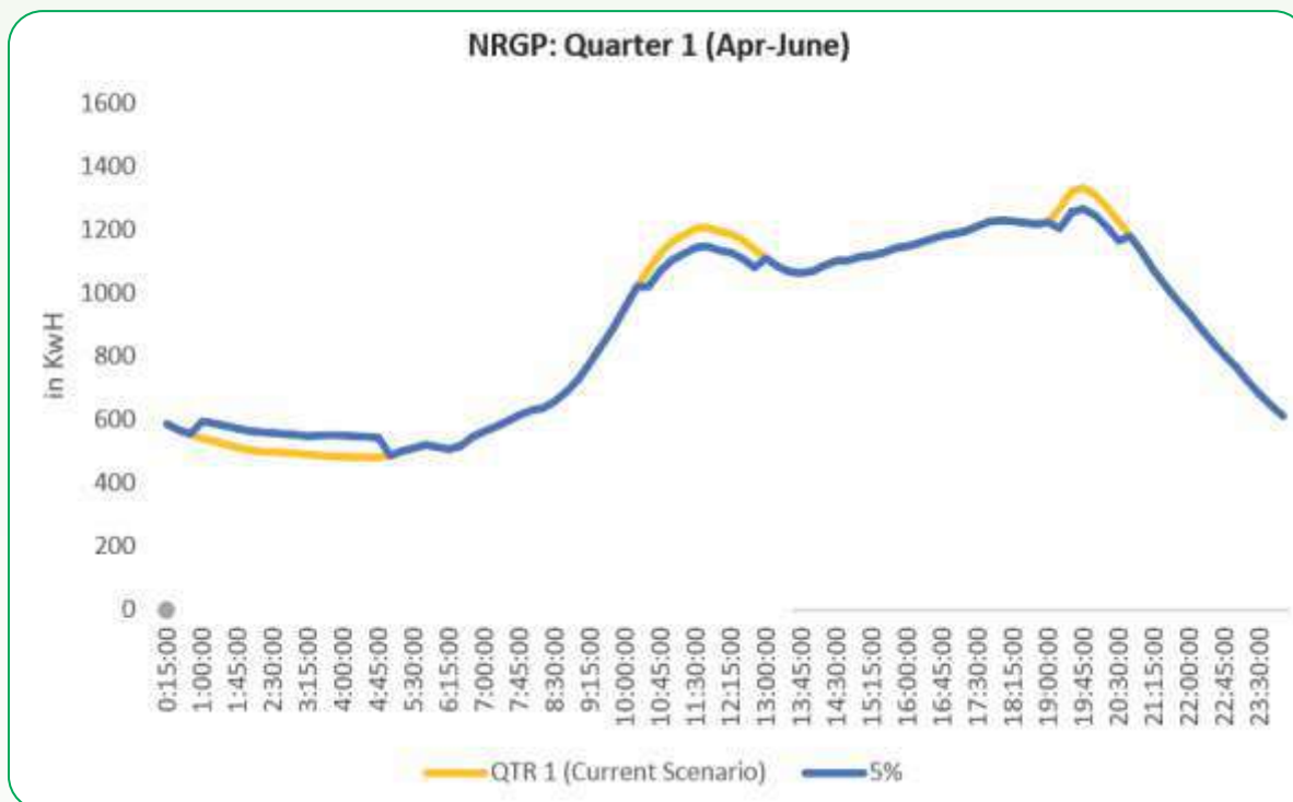
Figure 5-51: Change in NRGp night shift load curve in April-May-June due to 5% load shift
