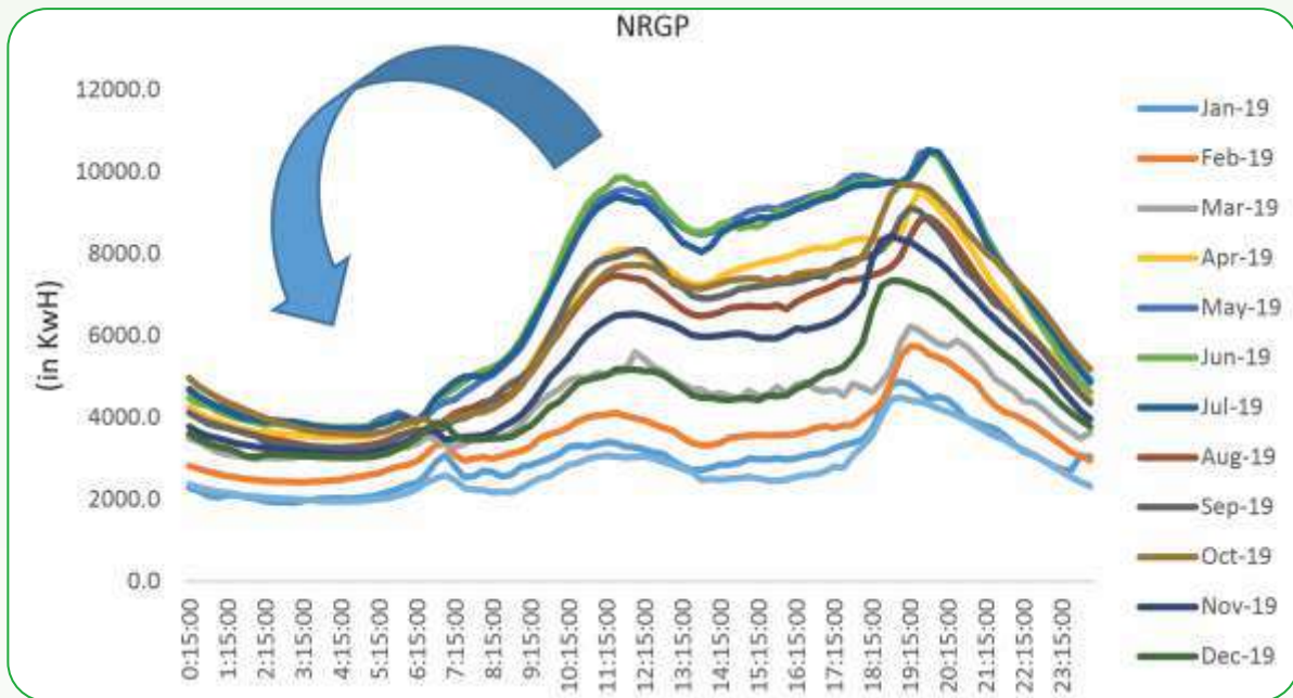
Figure 5-19: Dynamic pricing model- Shift in the load curve
