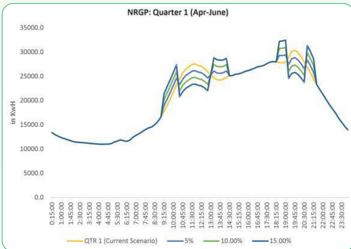
Figure 5-33: Change in NRG load curve in Apr-May-June due to 5%, 10% and 15% load shift
