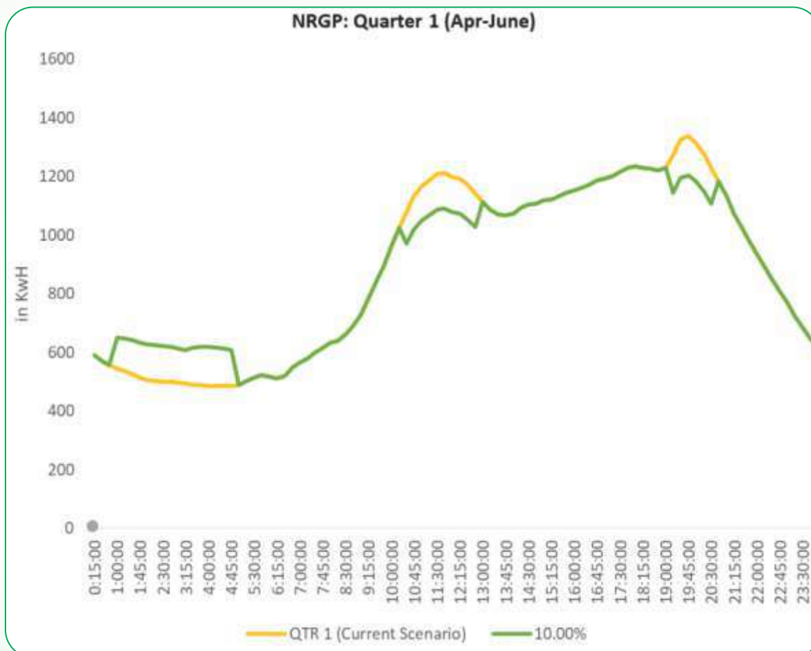
Figure 5-52: Change in NRGp night shift load curve in April-May-June due to 10% load shift
