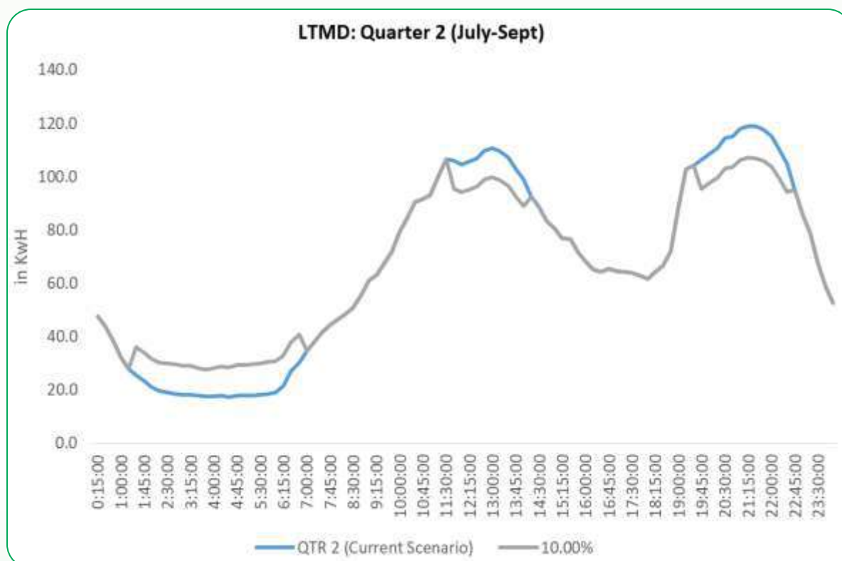
Figure 5-47: Change in LTMD night shift load curve in July-August-September due to 10% load shift
