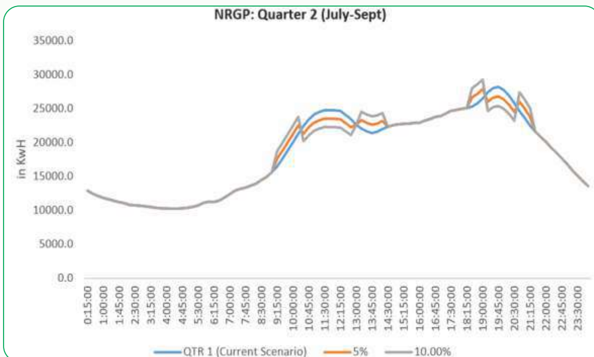
Figure 5-36: Change in NRGP load curve in July-Aug-Sept due to 5%, 10% load shift
