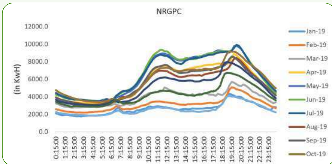
Figure 5-10: Consumption pattern for NRGPC consumers during Jan' 19- Jan' 20
