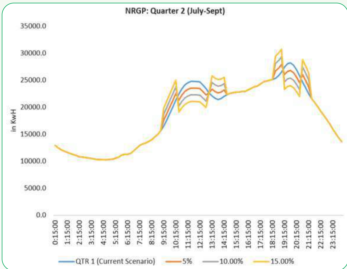
Figure 5-37: Change in NRG load curve in July-Aug-Sept due to 5%, 10% and 15% load shift
