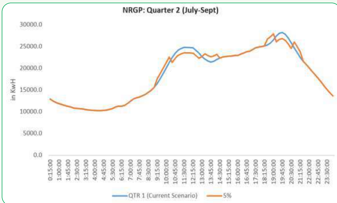
Figure 5-35: Change in NRGP load curve in July-Aug-Sept due to 5% load shift
