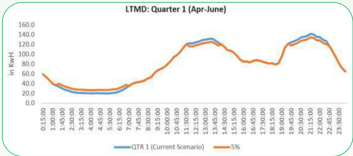
Figure 5-41: Change in LTMD night shift load curve in Apr-May-June due to 5% load shift
