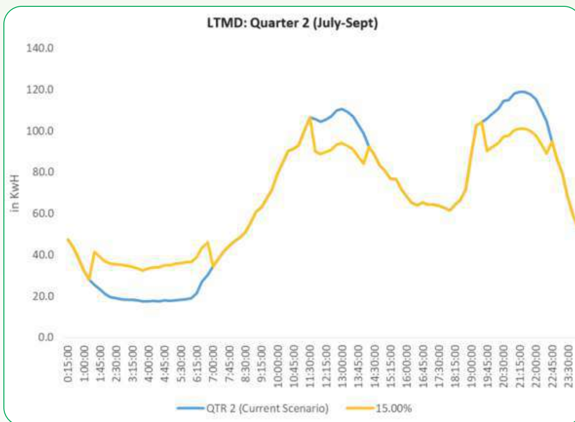
Figure 5-48: Change in LTMD night shift load curve in July-August-September due to 15% load shift
