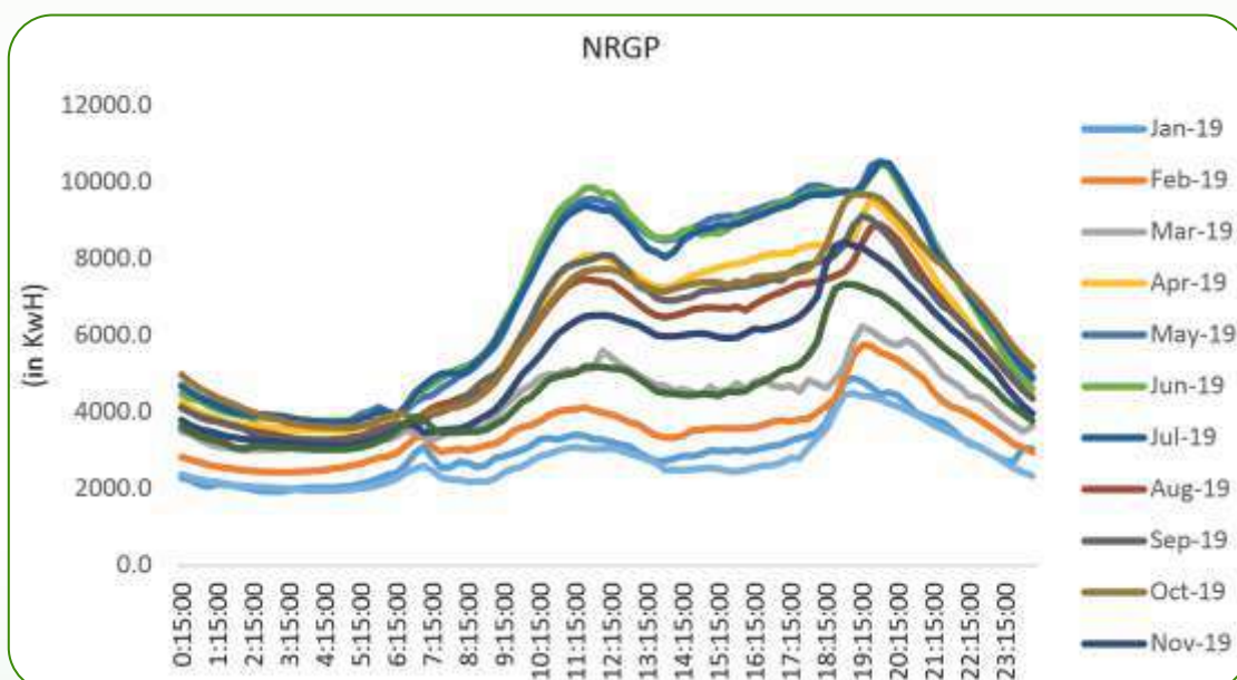
Figure 5-12: Consumption pattern for NRGPC consumers during Jan' 19- Jan' 20
