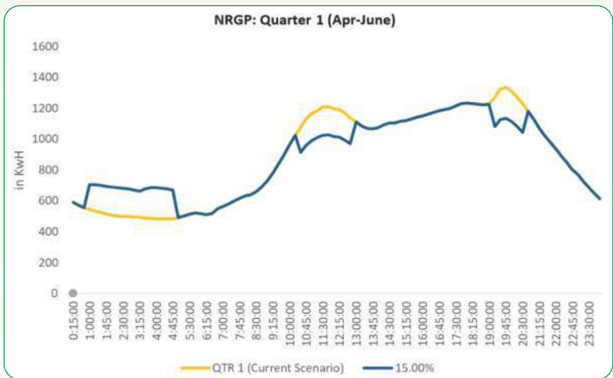
Figure 5-53: Change in NRGp night shift load curve in April-May-June due to 15% load shift
