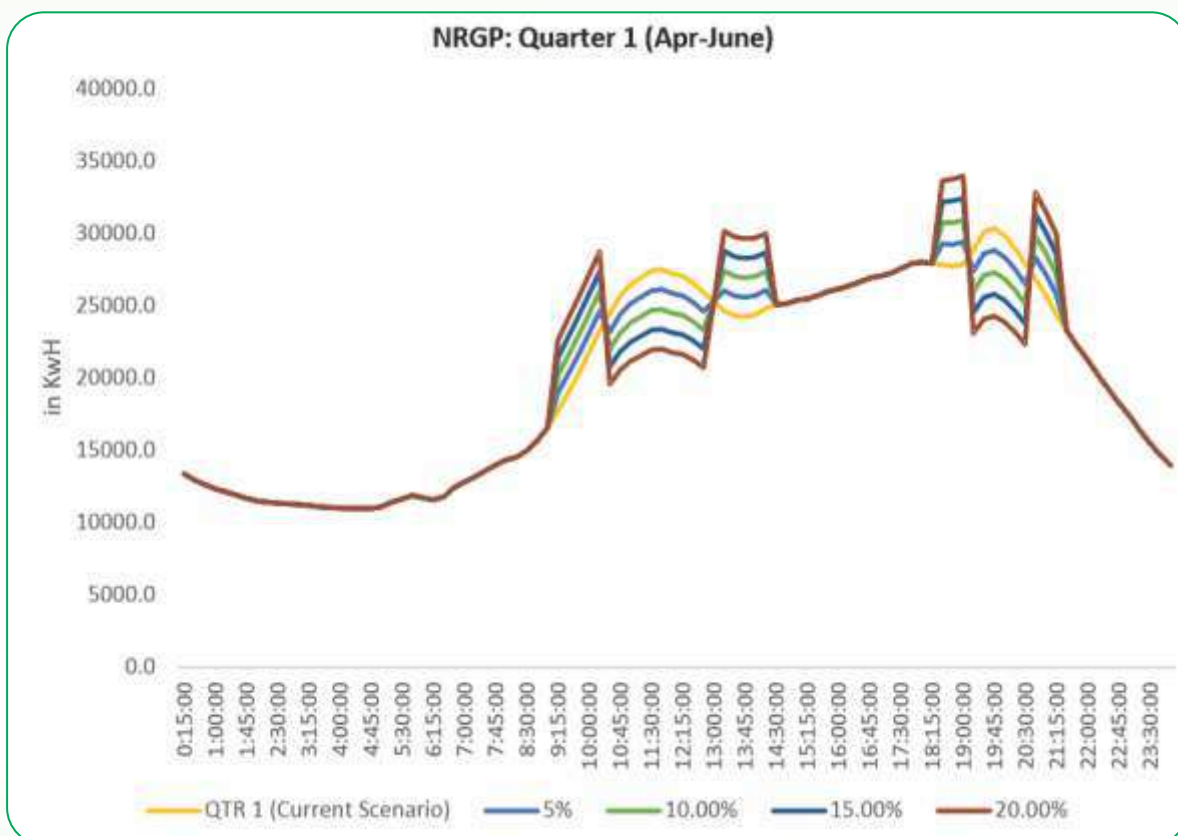
Figure 5-34: Change in NRG load curve in Apr-May-June due to 5%, 10%, 15% & 20% load shift
