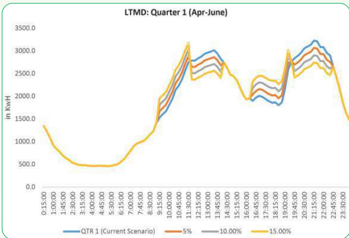
Figure 5-23: Change in LTMD load curve in Apr-May-June due to 5%, 10% and 15% load shift
