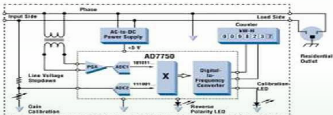
Figure 6-2: Analog Energy Meter
