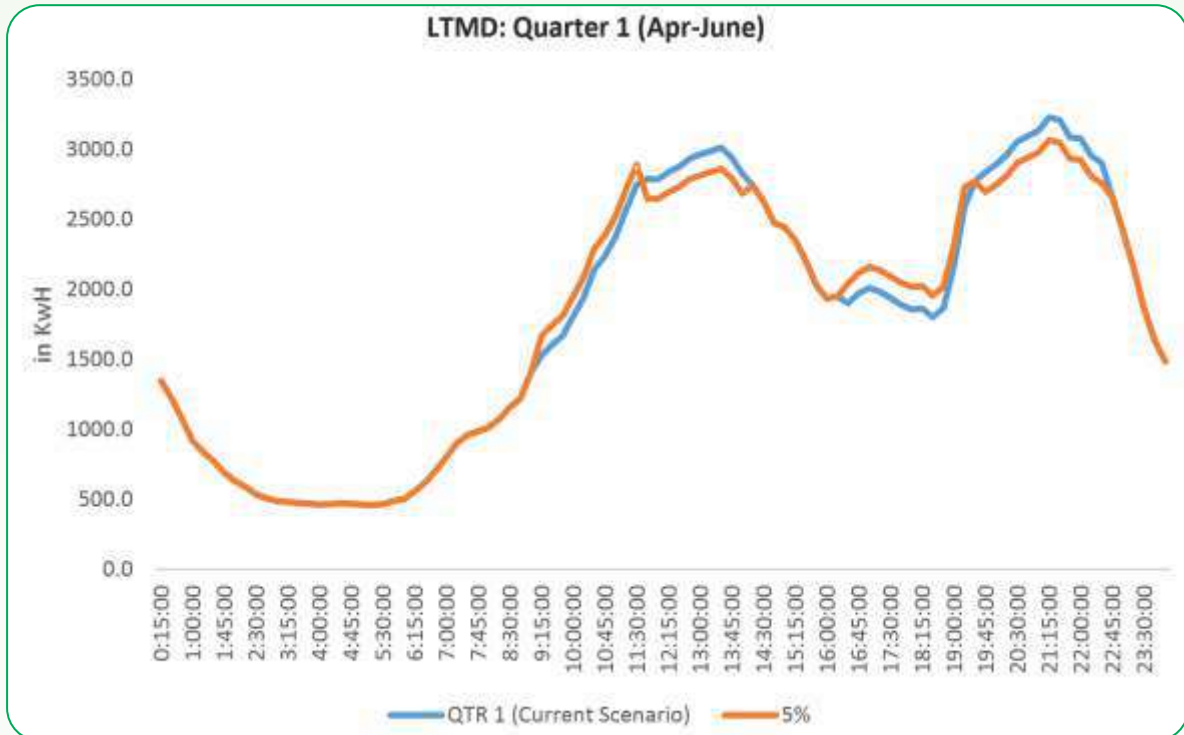
Figure 5-21: Change in LTMD load curve in Apr-May-June due to 5% load shift
