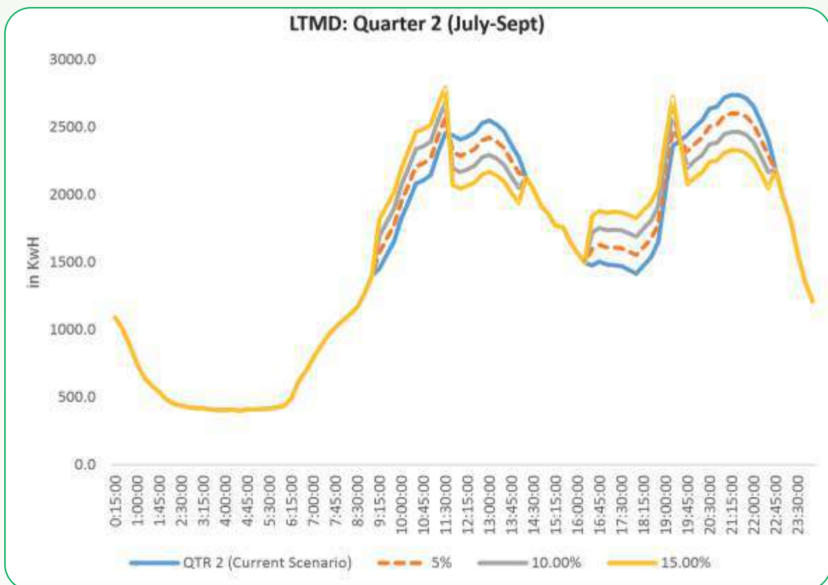
Figure 5-27: Change in LTMD load curve in July-Aug-Sept due to 5%, 10%, and 15% load shift
