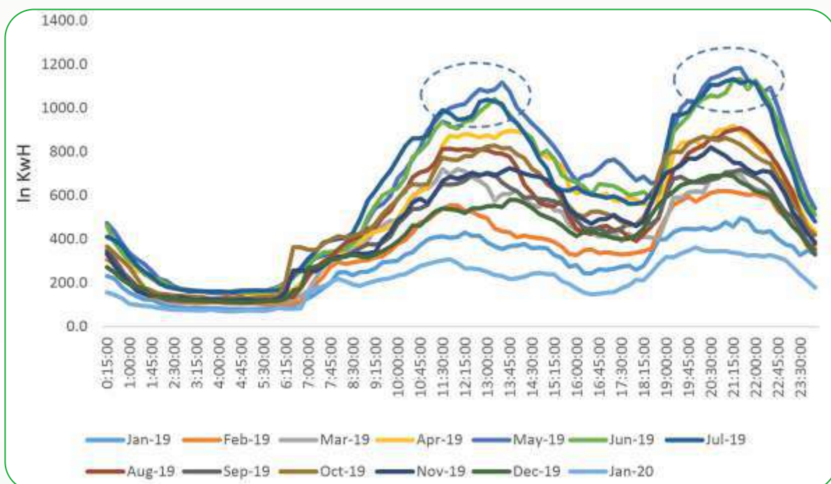
Figure 5-20: Load curve for LTMD consumers
