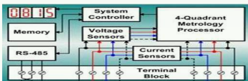
Figure 6-3: Digital energy meter
