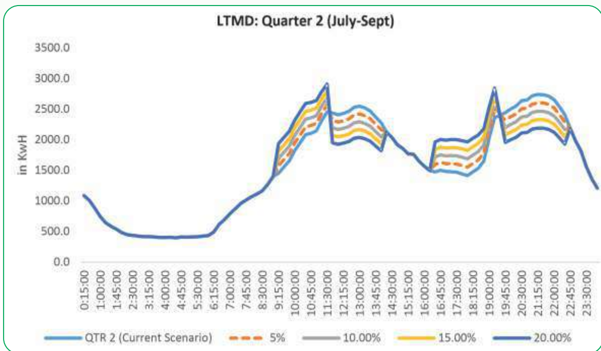
Figure 5-28: Change in LTMD load curve in July-Aug-Sept due to 5%, 10%, 15% and 20% load shift
