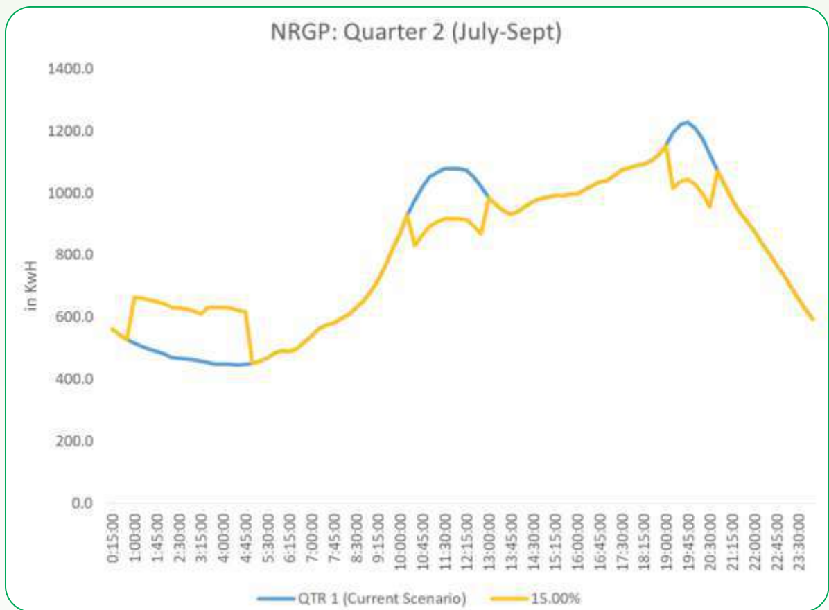
Figure 5-58: Change in NRG night shift load curve in July-August-September due to 15% load shift
