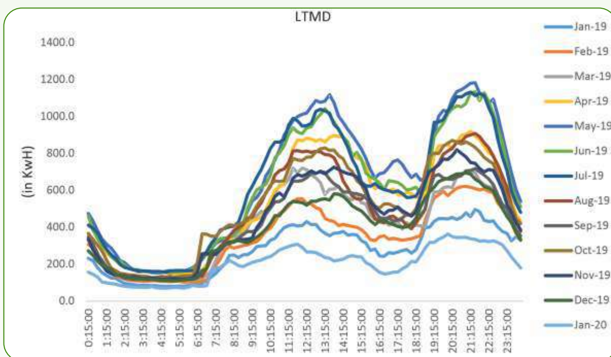
Figure 5-15: Consumption pattern for LTMD consumers during Jan' 19- Jan' 20
