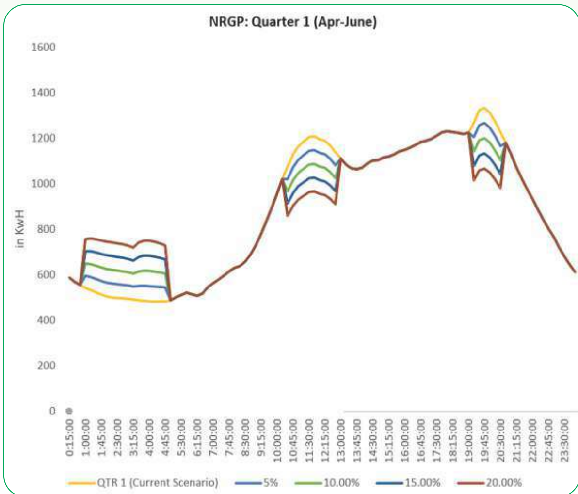
Figure 5-50: Load curve for NRGP night shift analysis consumers – First-quarter overall scenario
