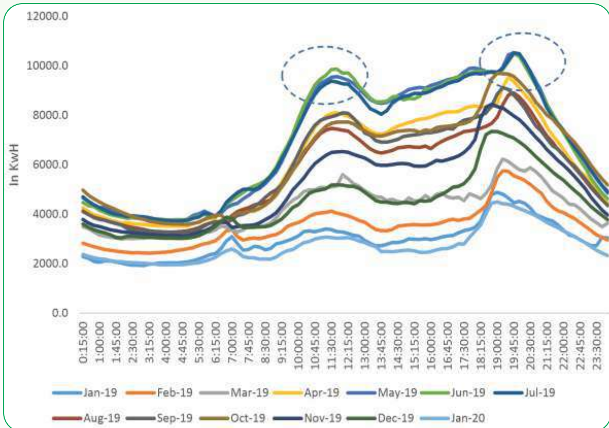
Figure 5-30: Load curve for NRGP consumers
