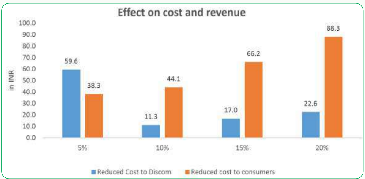
Figure 5-29: Financial impact on DISCOM and LTMD customers for the suggested ToU pricing above
