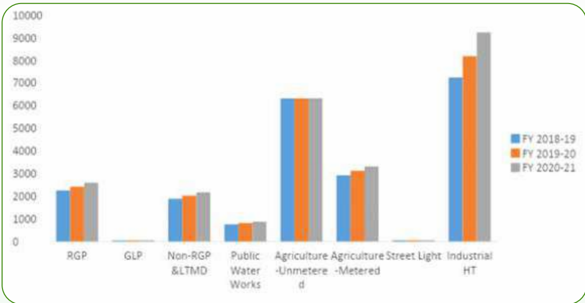
Figure 5-8: Projected energy sales for FY 2018-21 (in MUs)
