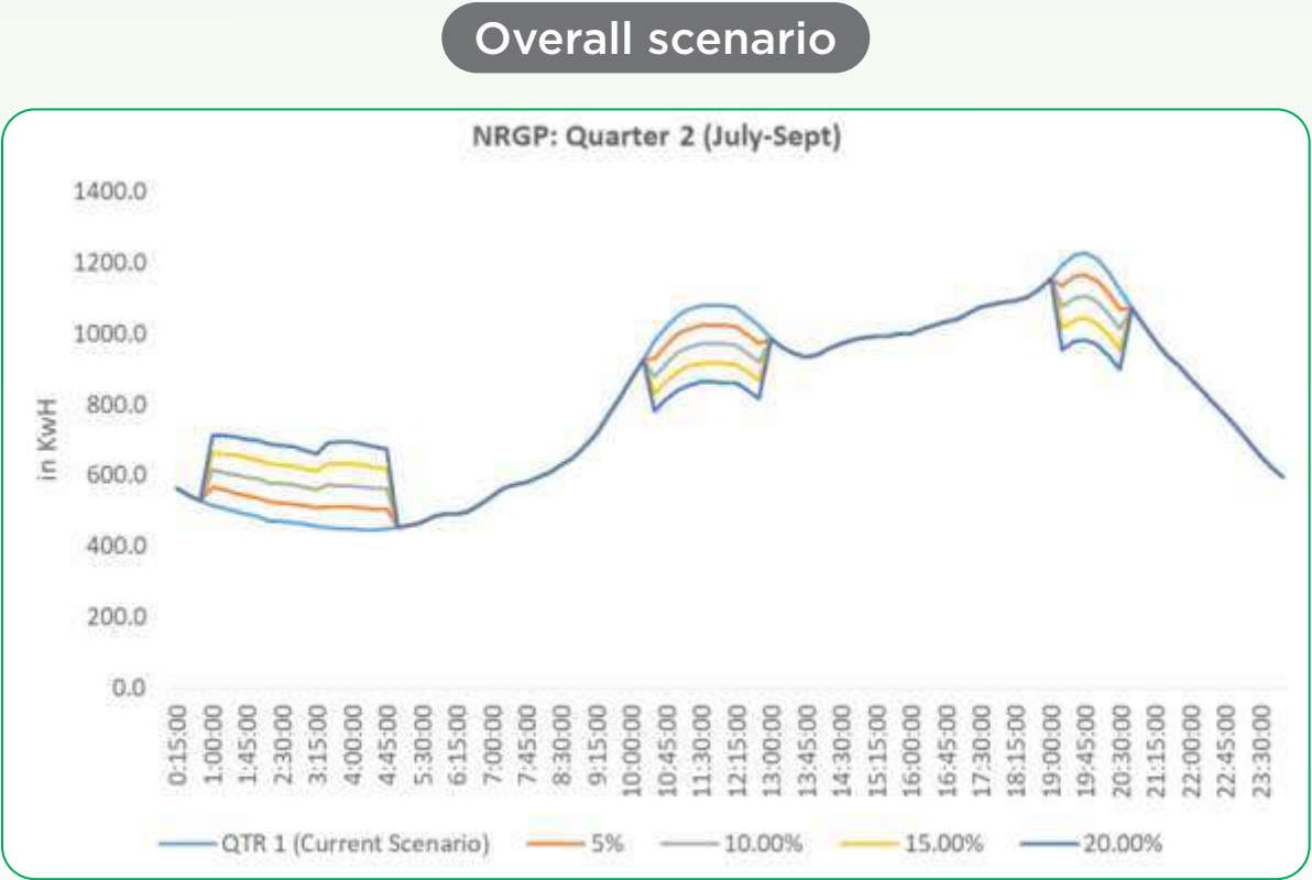
Figure 5-55: Load curve for NRGPs consumers night shift analysis – Second quarter overall scenario
