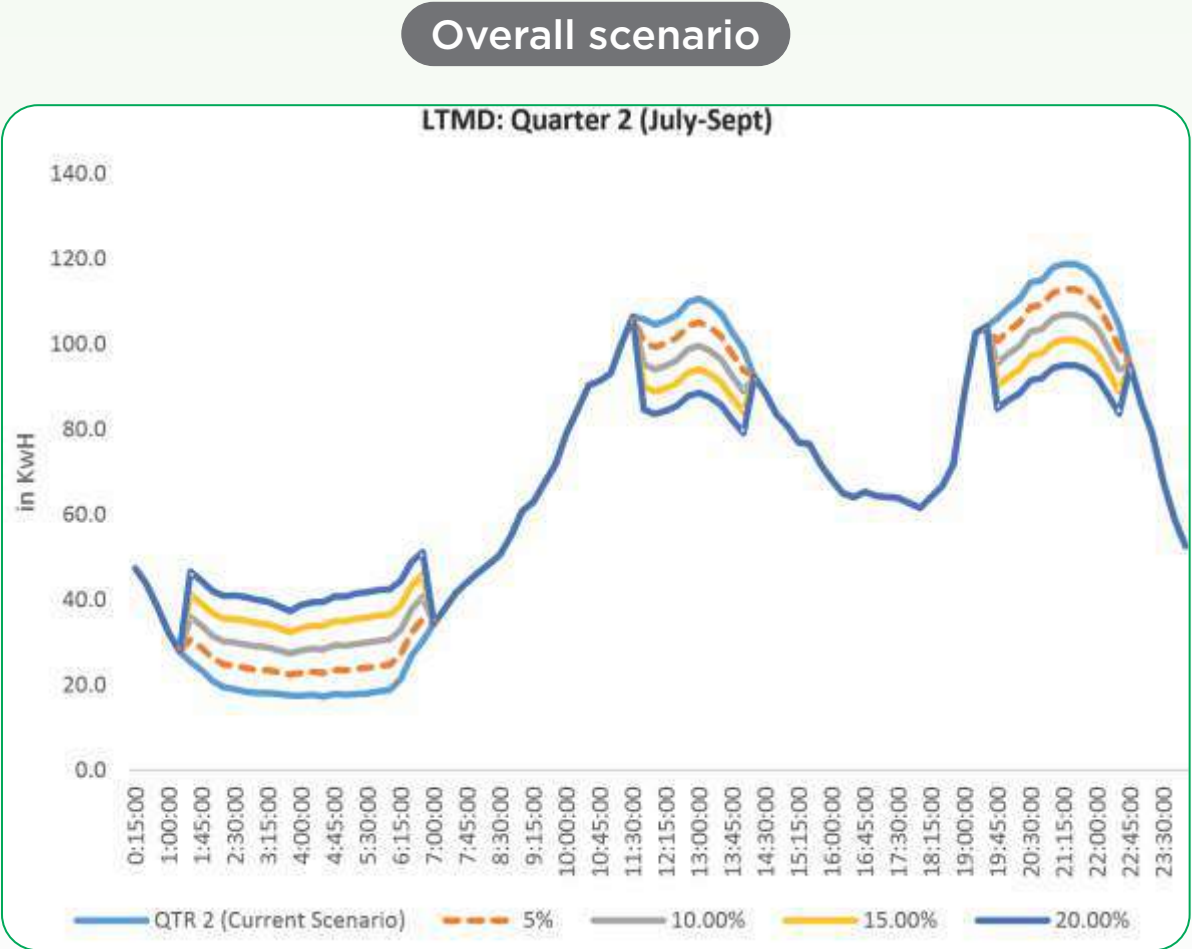
Figure 5-45: Load curve for LTMD night shift analysis consumers – Second quarter overall scenario
