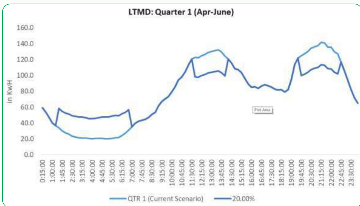
Figure 5-44: Change in LTMD night shift load curve in Apr-May-June due to 20% load shift
