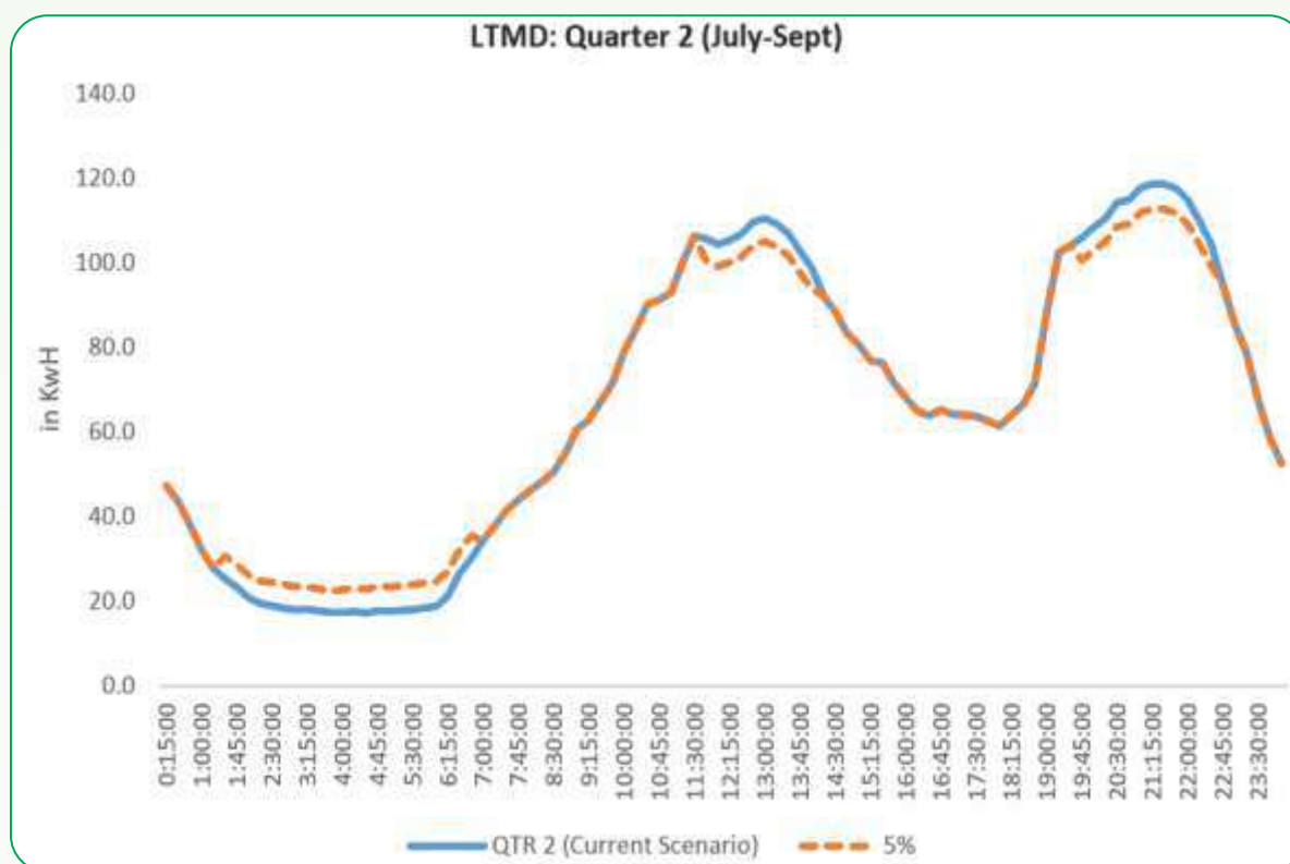
Figure 5-46: Change in LTMD night shift load curve in July-August-September due to 5% load shift
