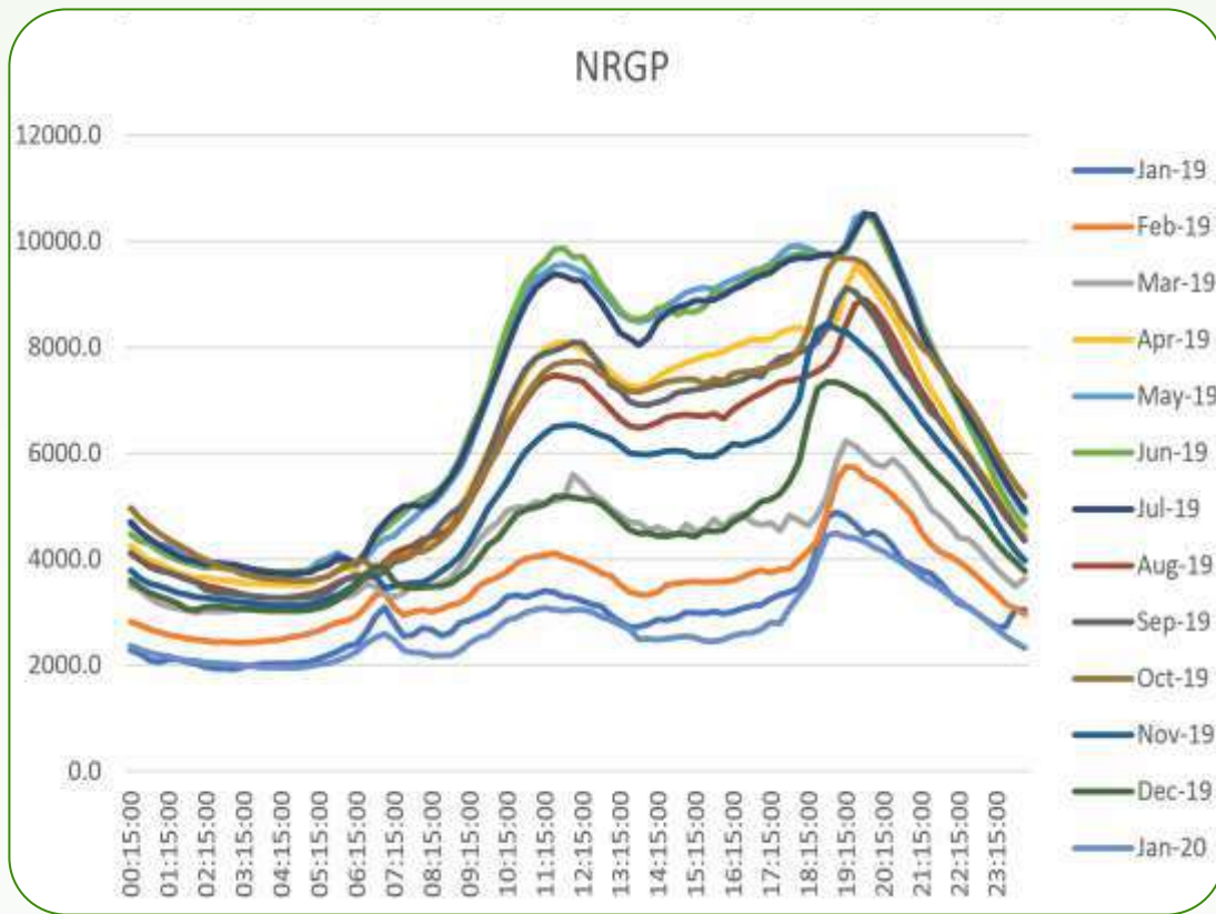
Figure 5-17: Consumption pattern for NRGF consumer in Naroda area (in KWh) (Jan-19 to Jan-20)
