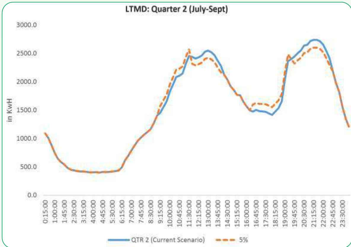
Figure 5-25: Change in LTMD load curve in July-Aug-Sept due to 5% load shift
