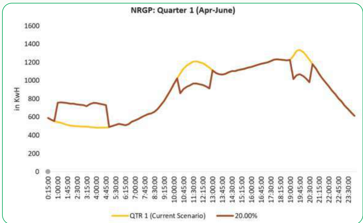
Figure 5-54: Change in NRGp night shift load curve in April-May-June due to 20% load shift
