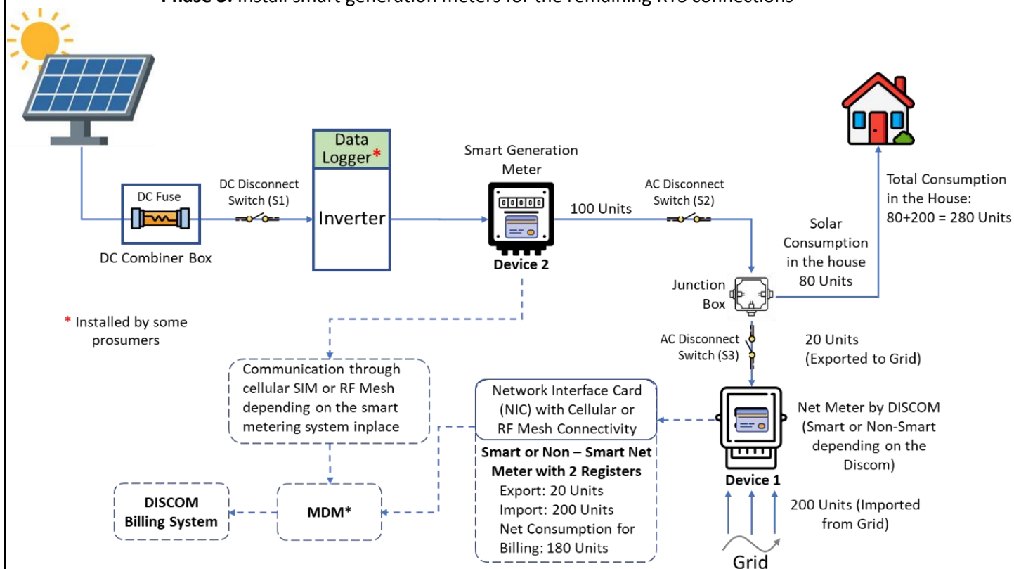
Figure 2: Proposed Generation Monitoring System with Smart Generation Meter for Existing RTS
