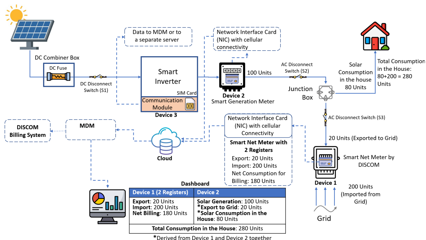
Figure 4: Proposed Generation Monitoring System with Smart Generation Meter for New RTS Connections where Smart Metering has Cellular Communication System
