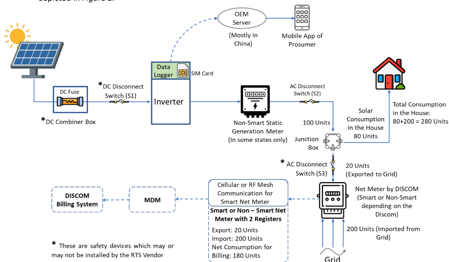
Figure 1: Present RTS Connection and Generation Data Monitoring System by Prosumers 1
