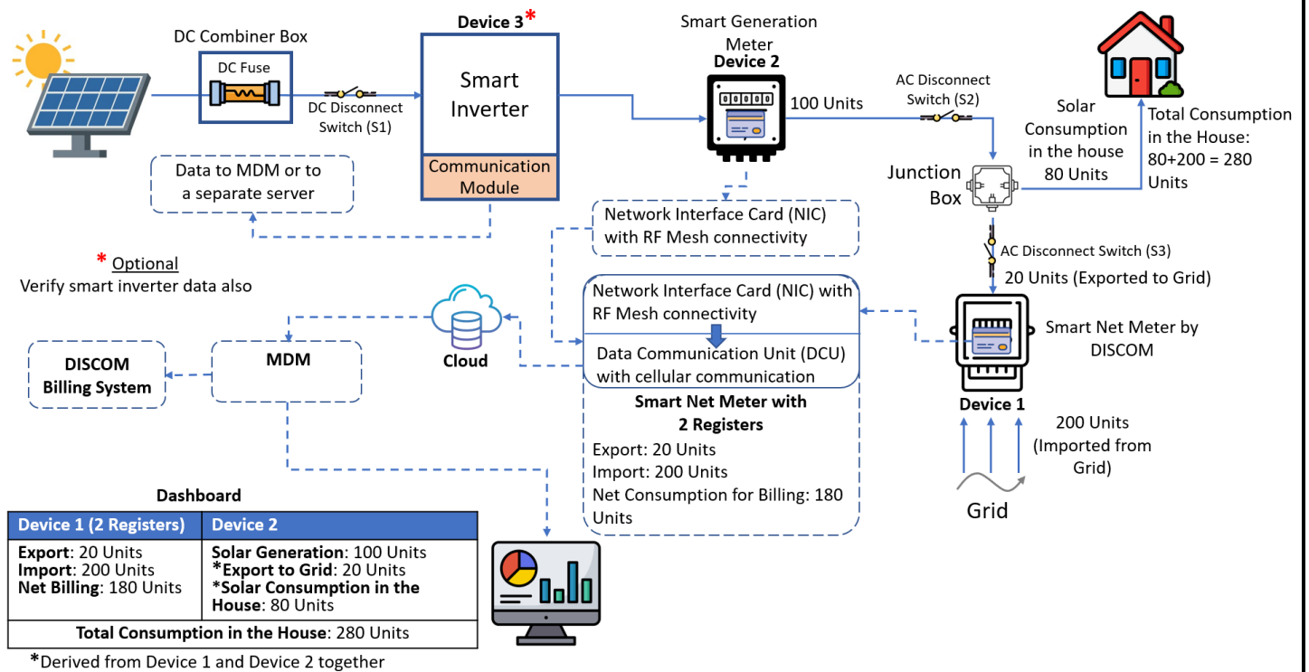
Figure 3: Proposed Generation Monitoring System with Smart Generation Meter for New RTS Connections where Smart Metering has RF Mesh for Last Mile Connectivity
