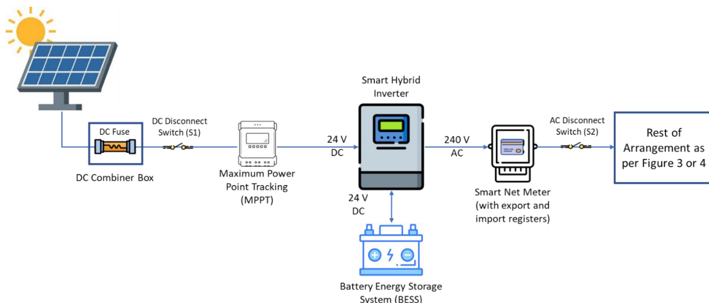
Figure 5: Proposed Connection Arrangement for RTS with MPPT 9 and Hybrid Inverter and Battery Energy Storage System (BESS)
